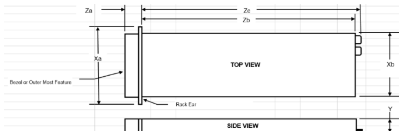
Figure 36. Chassis dimensions
