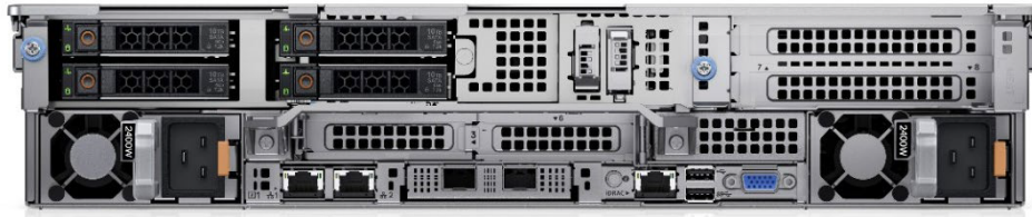
Figure 12. Rear view of the R750 with 4x 2.5 inches storage drives, 4x PCIe Gen4 slot and Hot-plug BOSS
